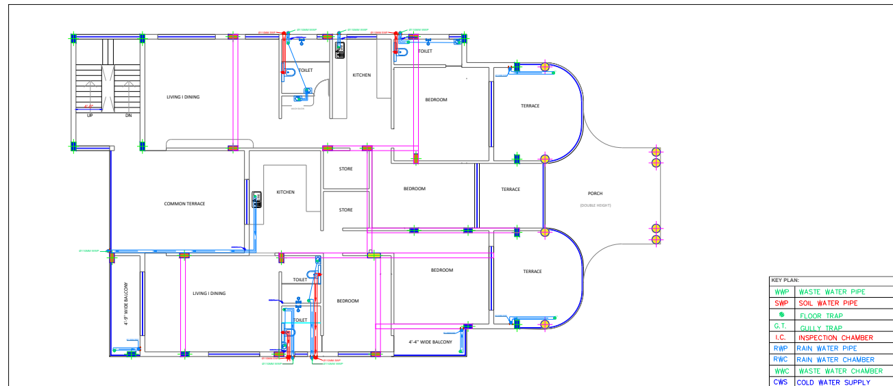
← MAIN ROAD → FIRST FLOOR PLAN SLAB AREA = 3170 + 800 (BALCONY) (POORHALL)
