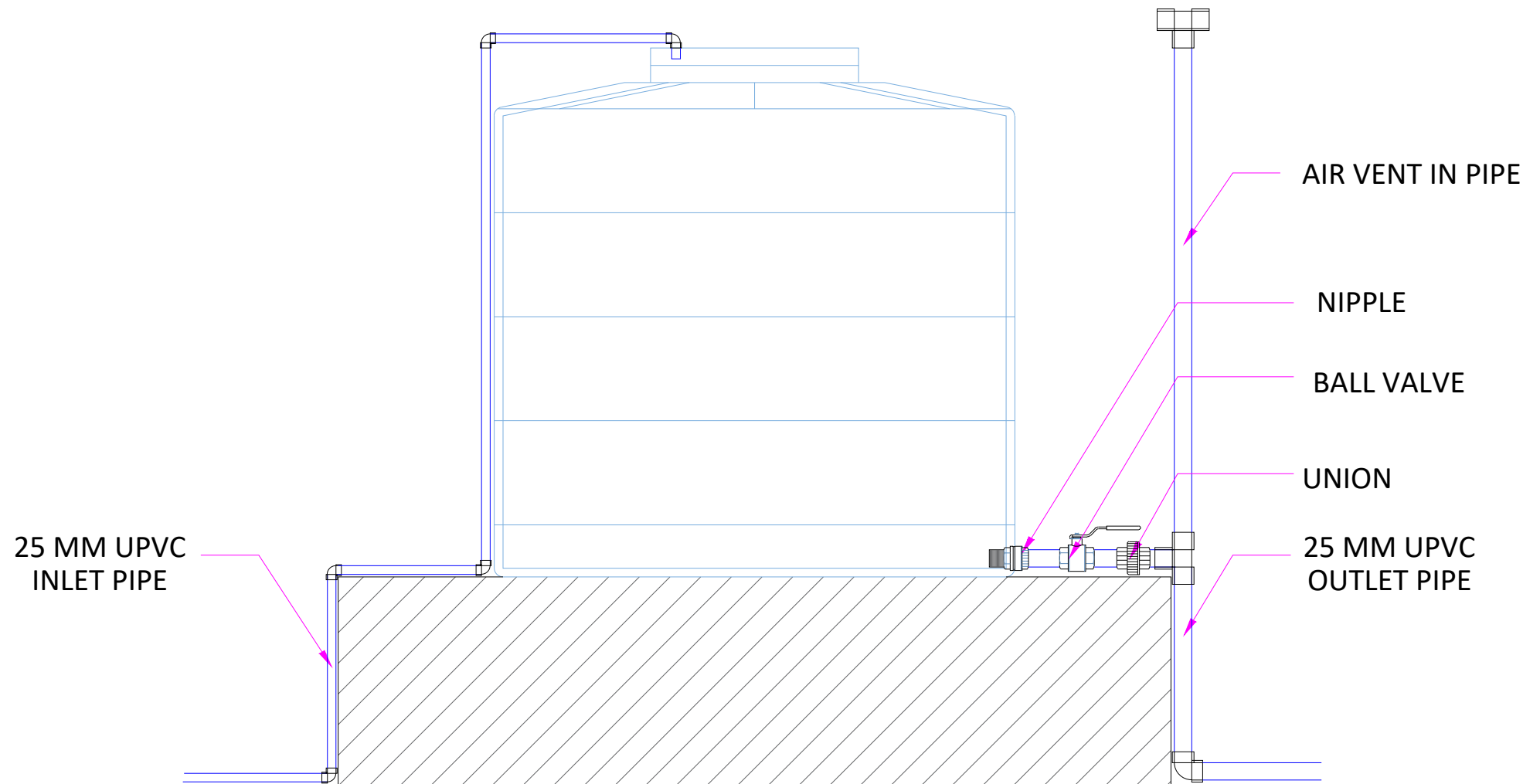
OVER HEAD TANK LAYOUT
