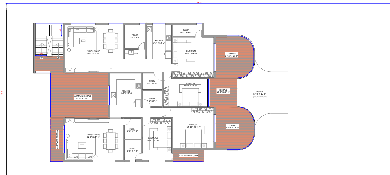
← MAIN ROAD → FIRST FLOOR PLAN SLAB AREA = 11761.60 SQ. FT. (100% TYP.)
