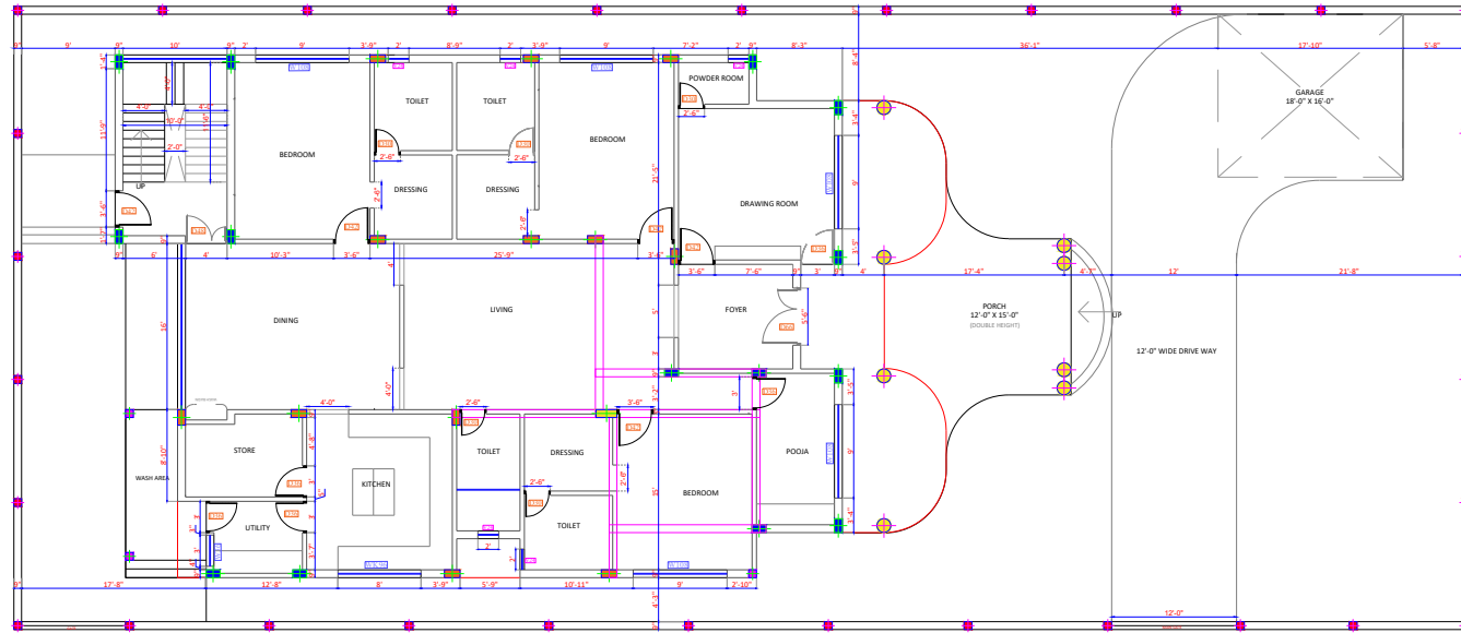
← MAIN ROAD → GROUND FLOOR PLAN SLAB AREA = 3170 + 400 (H.F.) (DOOR + STAIRS)
