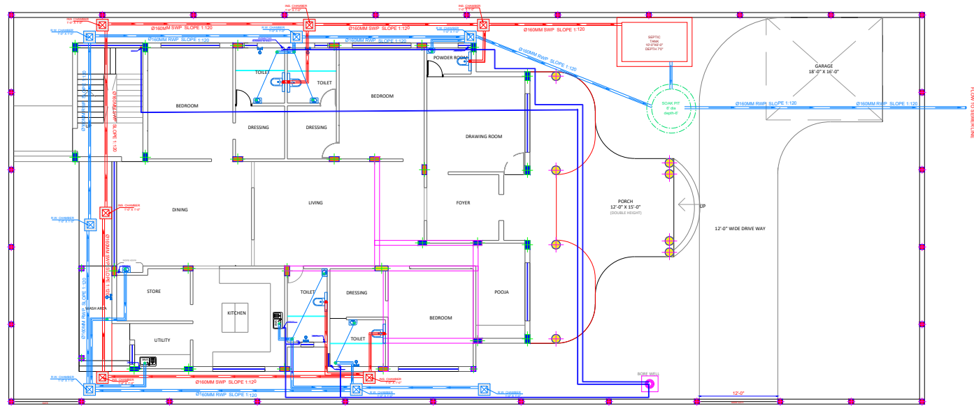
← MAIN ROAD → GROUND FLOOR PLAN SLAB AREA = 3170 + 800 (BALCONY) (POORHALL)
